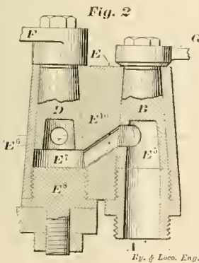
SAND BLOWER AND BRAKE ATTACHMENT.
